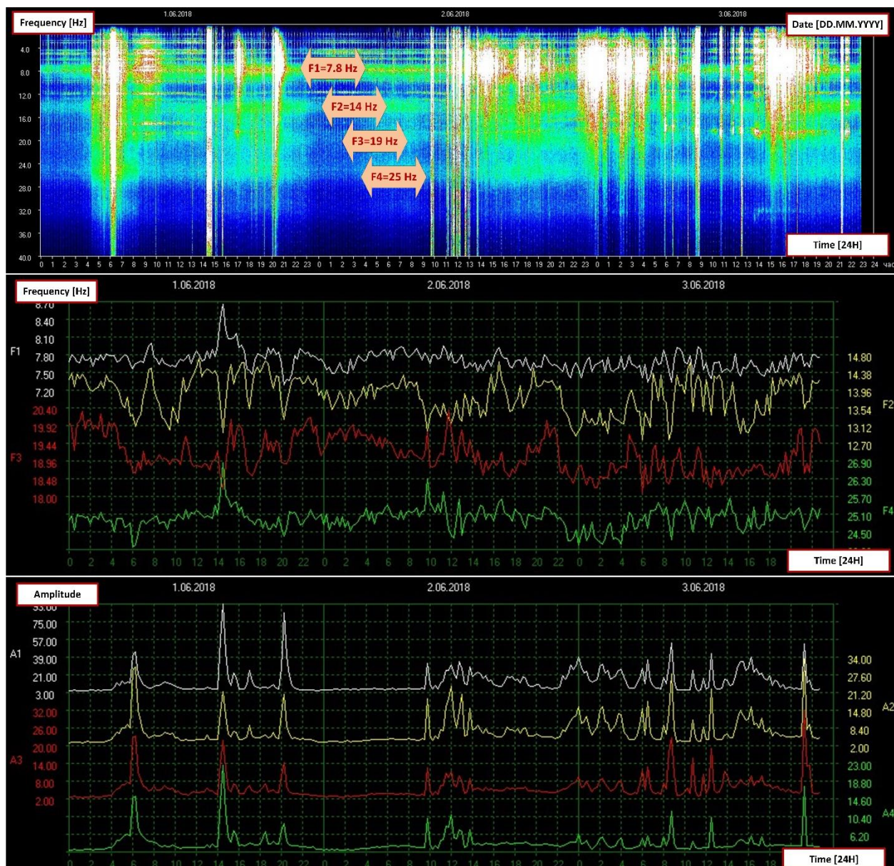
Fig. 2. Live monitoring of the Schumann resonance first four modes at the Tomsk Space Observing System station ( http://sosrff.tsu.ru/?page_id=7 ) in Siberia, Russia. You see a strong correlation between frequency/amplitude of the Schumann frequencies and a lightning activity in the area.
